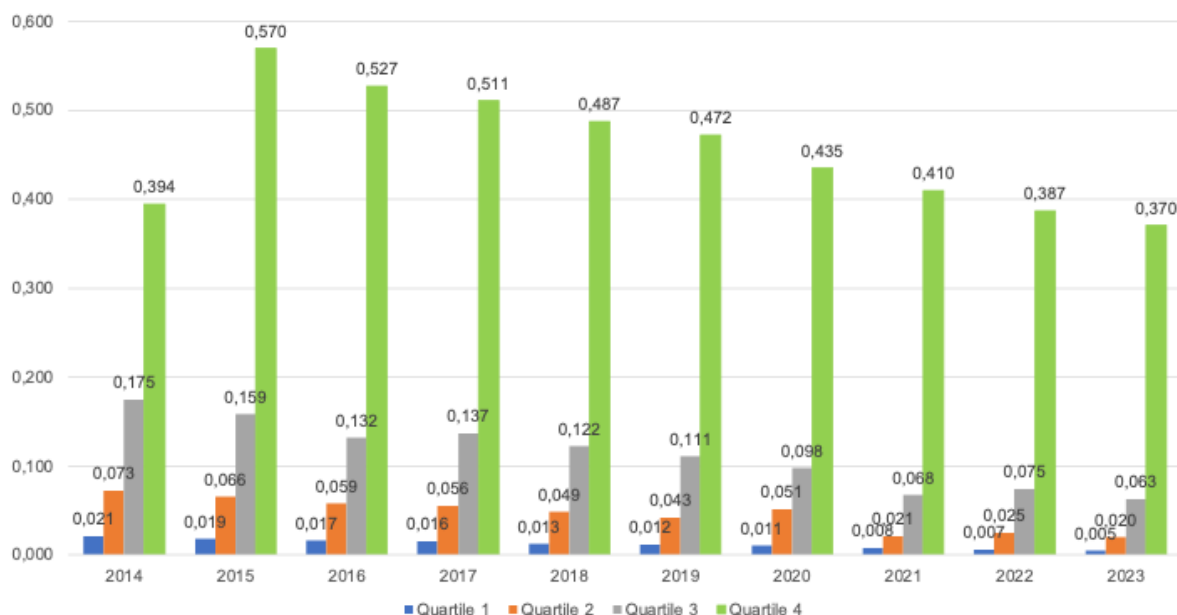
Fig. 3. Annual concentration ratios (CR) for each quartile of LCs.
